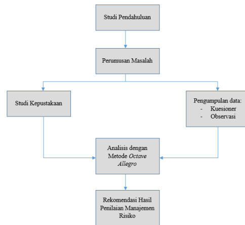
Gambar 4. Alur Penelitian
