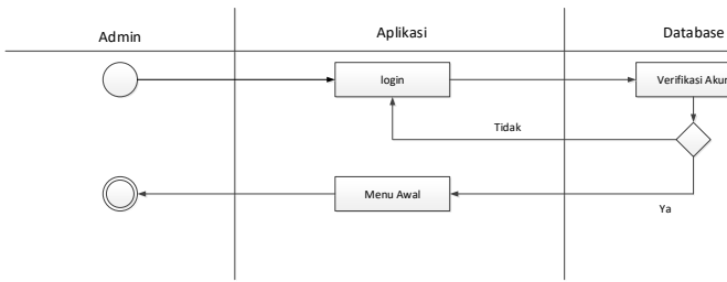
Gambar 7. Activity Login
