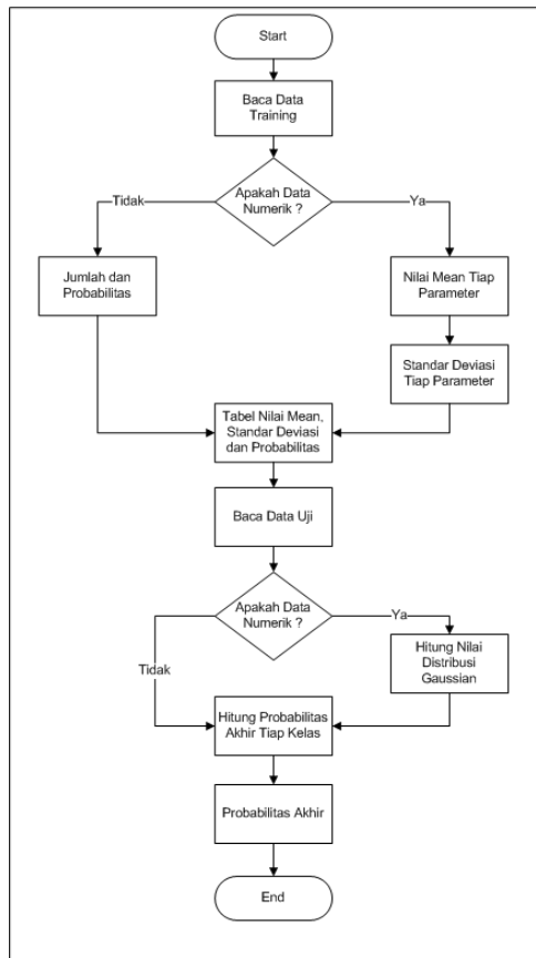
Gambar 1 Alur Naïve Bayes Classifier
